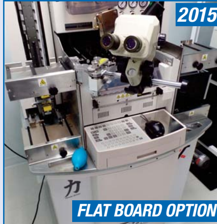
K&S ICONN PS HIGH PERFORMANCE WIRE BONDER
